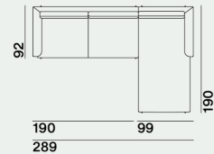
01FLAC3 (1FLAD3SX + 1FLACHLMDX), 02FLAC3 (2FLAD3SX + 2FLACHLMDX)
